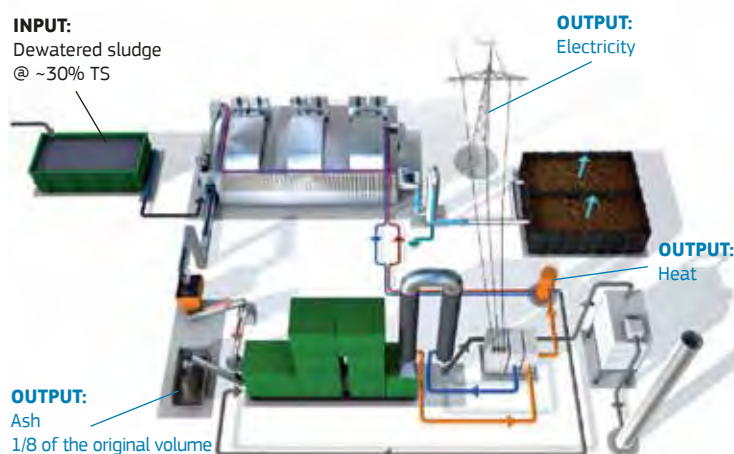
SLUDGE2ENERGY process diagram
