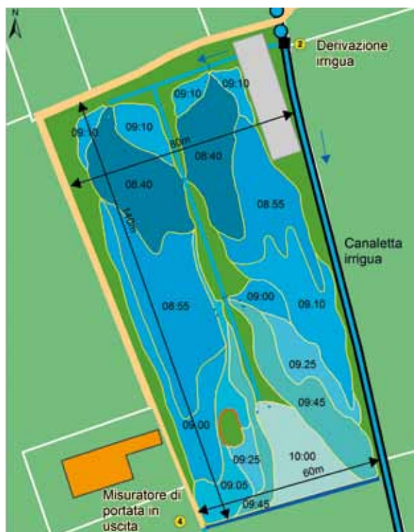
The test field and the progressive water distribution during the initial phases of water provision at the Busta site
